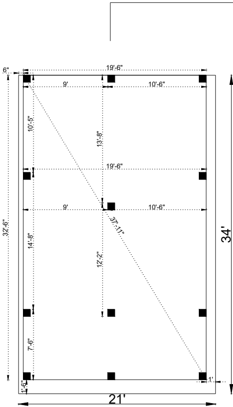
COLUMN MARKING
