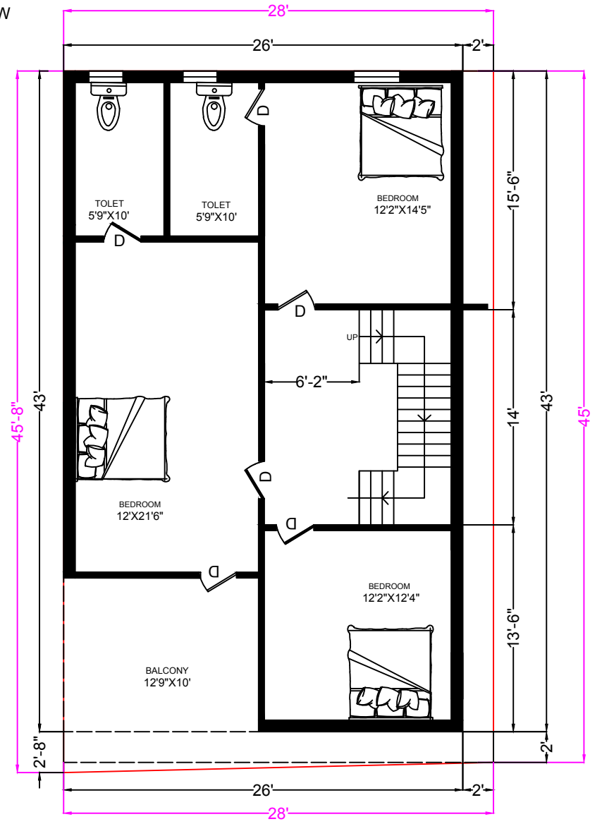
FIRST FLOOR
