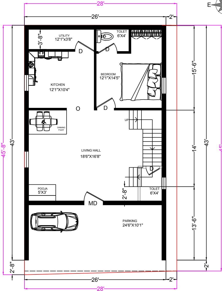
GROUND FLOOR
