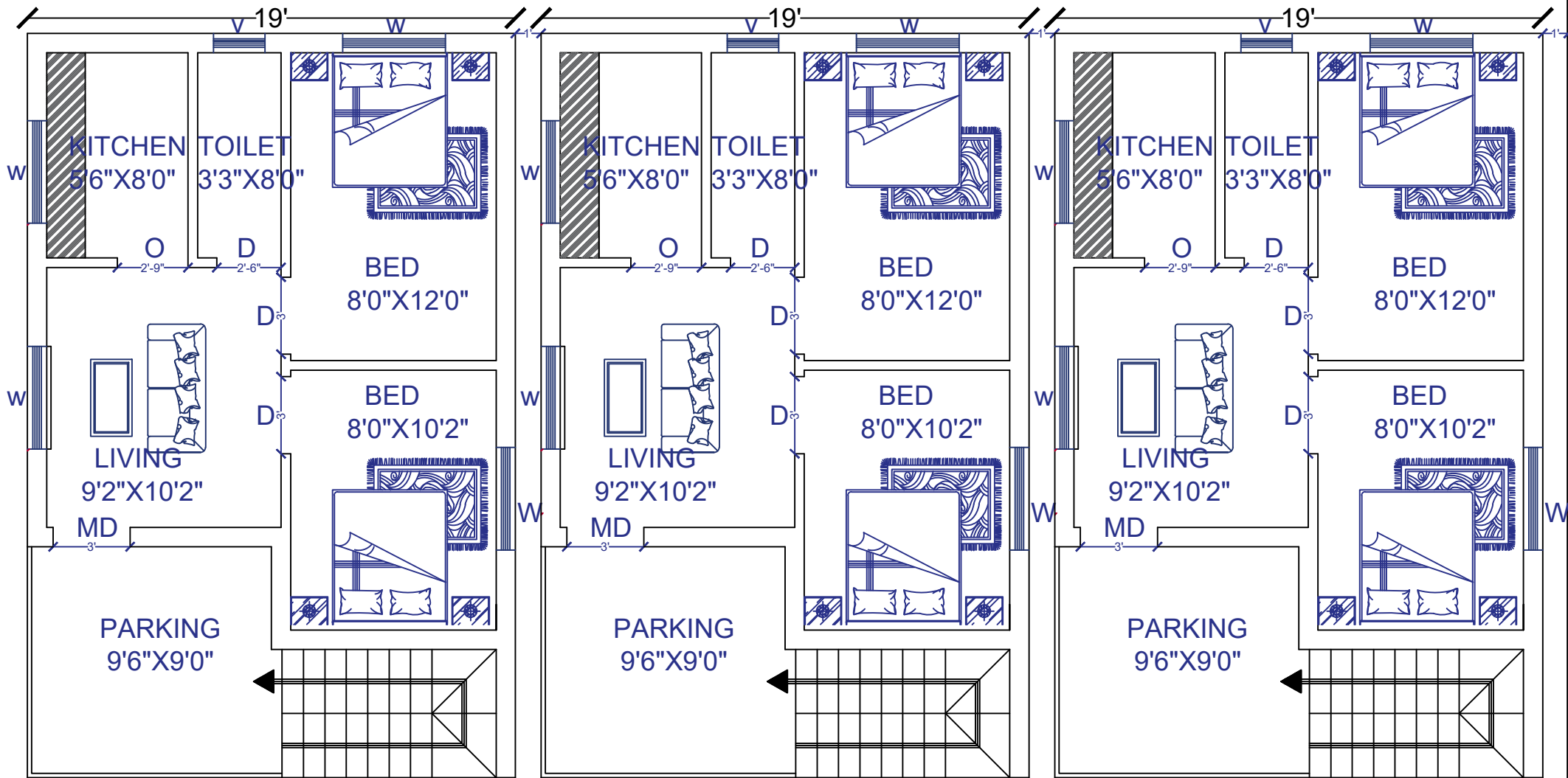
GROUND FLOOR PLAN PLINTH AREA - 551 SQ.FT (EACH ONE)
